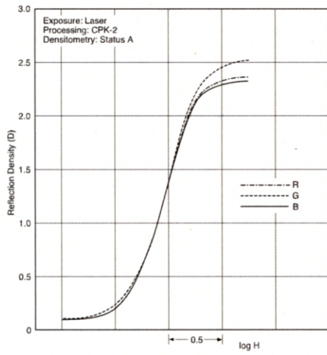
Characteristic Curves
